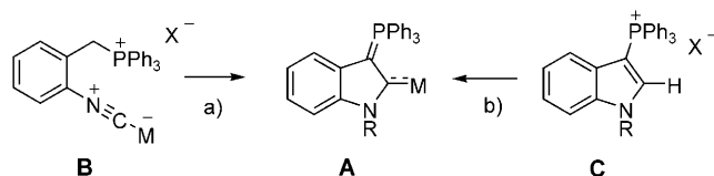
Scheme 1. Known entries into metal-AYC complexes: a) M = [\text{PtCl}_2(\text{PR}_3)] , \text{Et}_3\text{N} (excess), R = \text{H} ; or M = [\text{W}(\text{CO})_5] , \text{Na}[\text{N}(\text{SiMe}_3)_2] , R = \text{H} ; b) M = [\text{Rh}(\text{cod})\text{Cl}] , mesityllithium, R = \text{Me} ; or M = [\text{Pd}(\text{allyl})] , t\text{BuOK} , R = \text{Me} . cod = 1,5-cyclooctadiene.
