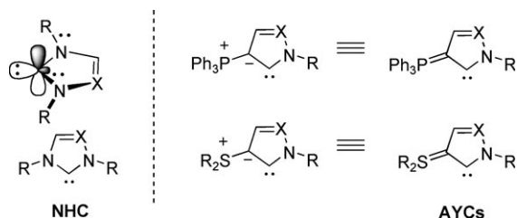
Figure 1. Basic structure of an N-heterocyclic carbene (NHC) as a prototype singlet carbene stabilized by two flanking amino groups ( X = \text{CH}, \text{N} ; R = \text{alkyl, aryl} ). The formal replacement of one NR unit by an ylide leads to an archetypal (amine)(ylide)carbene (AYC) species.
